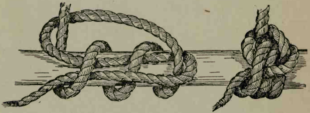
FIG. 54.—Gaff-topsail halyard bend.
